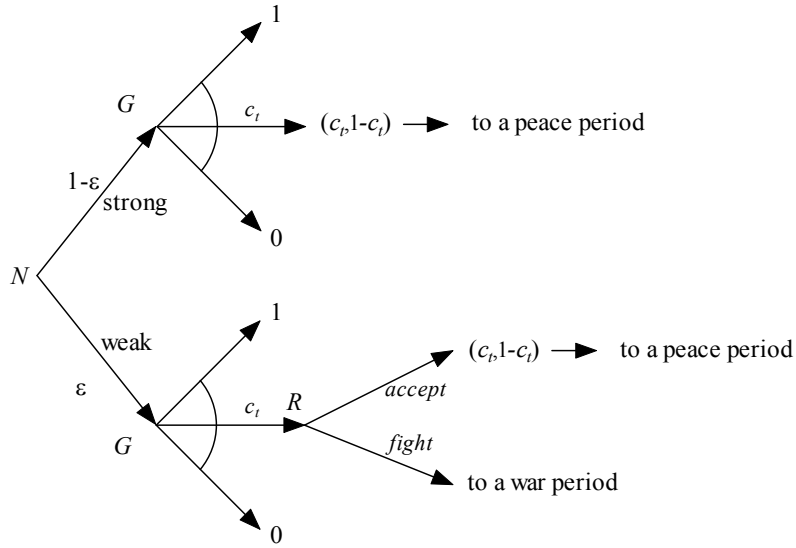
Figure 1: A model of sessionist civil wars.
